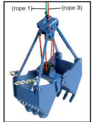
05. fix and rope-up respectively the grabber ropes (1) and (3)
