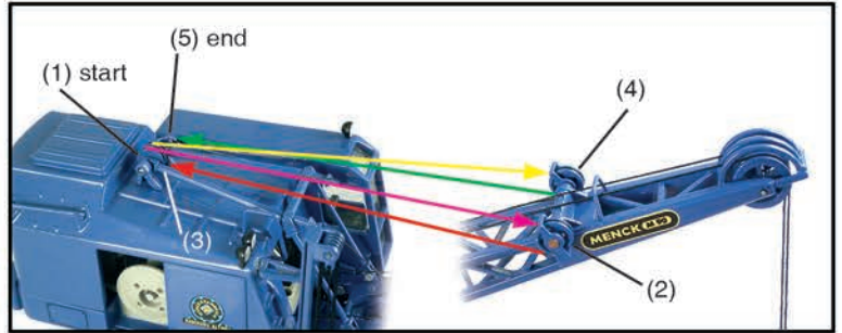
04. rope-up the lattice mast rope (2)
